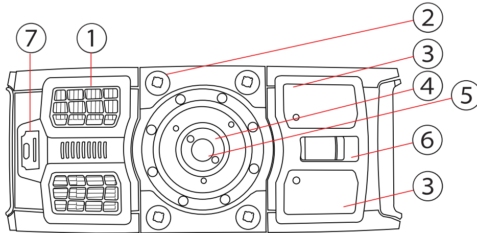
Figure 4-4 Bottom View of the FARO Focus Premium
