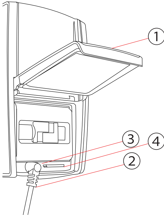
Figure 4-2 Battery Side of the FARO Focus Premium
