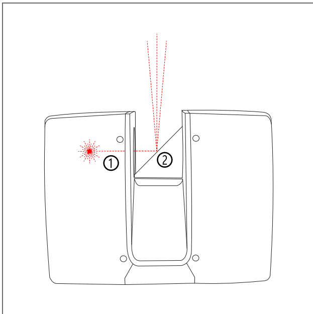
Figure 2-2 Laser Deflection
