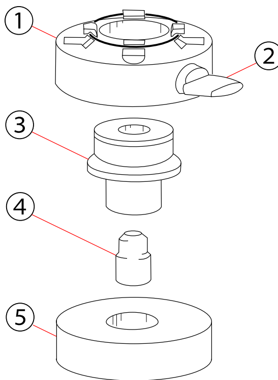
Figure 5-7 Quick release parts
