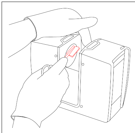
Figure 8-10 Cleaning sensor cover with pad and isopropyl alcohol or cleaning fluid
