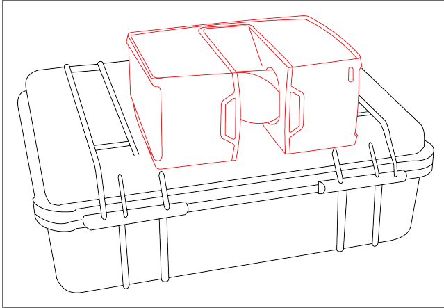
Figure 8-12 Transport box with laser scanner turned and laid on top, with the mirror module facing outwards
