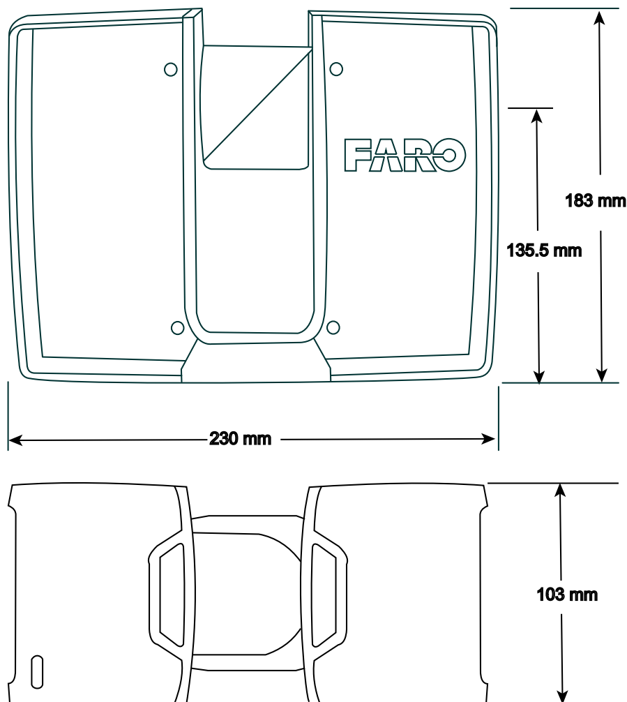
Figure 9-1 Scanner Dimensions
