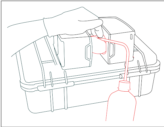
Figure 8-14 Cleaning mirror module or sensor cover
