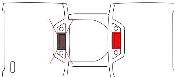
Figure 4-7 : Accessory bay for the status indicator with covers
